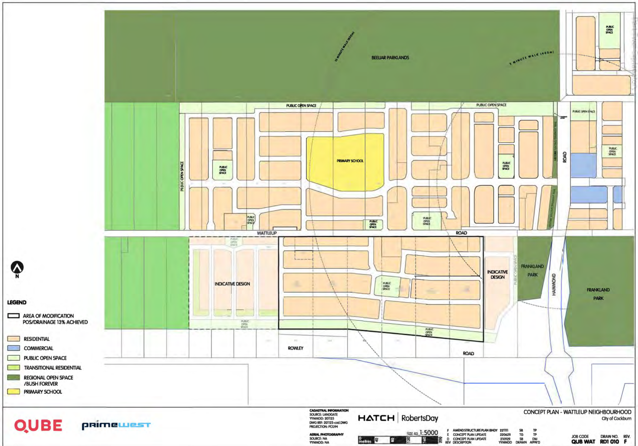
Figure 9 - Neighbourhood Concept
